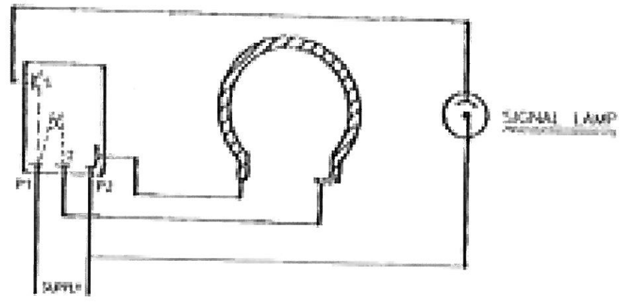
WIRING DIAGRAM, WIRING DIAGRAM, ELECTRICAL CONNECTIONS
